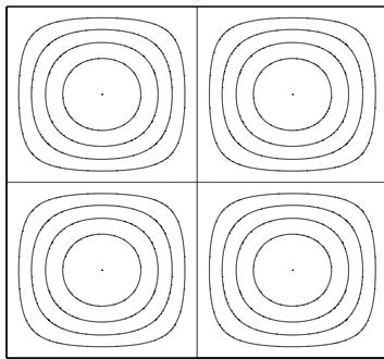
FIGURE 1. Streamlines of the cellular flow u_{\text{cell}} .
