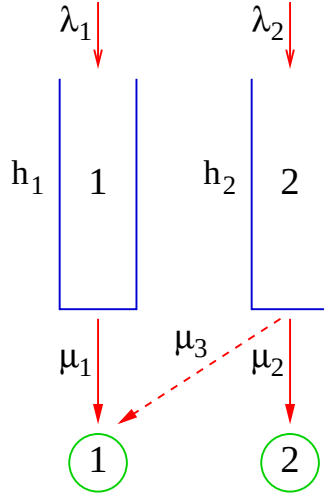
FIG 3. Two “trees” connected via a single non-basic activity
