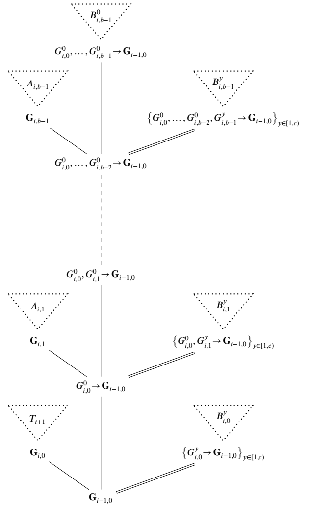
Fig. 3. The structure of the tree T_i , for i < a-1 .
