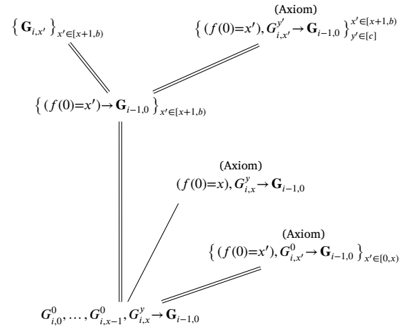
Fig. 4. The structure of the tree B_{i,x}^y .
