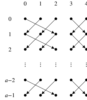
Fig. 1. The CNF formula \Gamma_{a,b} is visualized as a [a] \times [b] array of variables. Shown with b = 5 . Implications (actually, reverse implications) are shown by arrows. E.g., in the figure f(0) = 2 , f(1) = 0 , etc. The same f is used for all rows.
