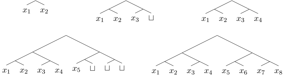
Figure 1: Five encodings of words by binary trees: \nu_t(x_1x_2) , \nu_t(x_1x_2x_3) , \nu_t(x_1 \dots x_4) , \nu_t(x_1 \dots x_5) and \nu_t(x_1 \dots x_8) .
