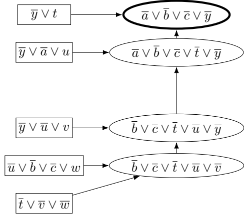
(b) The trivial resolution derivation of \bar{a} \vee \bar{b} \vee \bar{c} \vee \bar{y} (written bottom-up).
