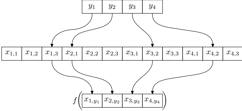
Figure 7.21. Illustration of lifted function (for \ell = 3 , m = 4 , and y = (3, 1, 2, 2) ).
