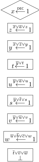
(a) The unit propagations triggered by setting x true.
