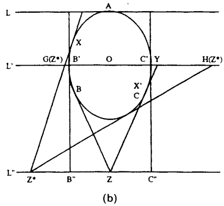
Fig. 1. Construction of \{A, B, C\} .
