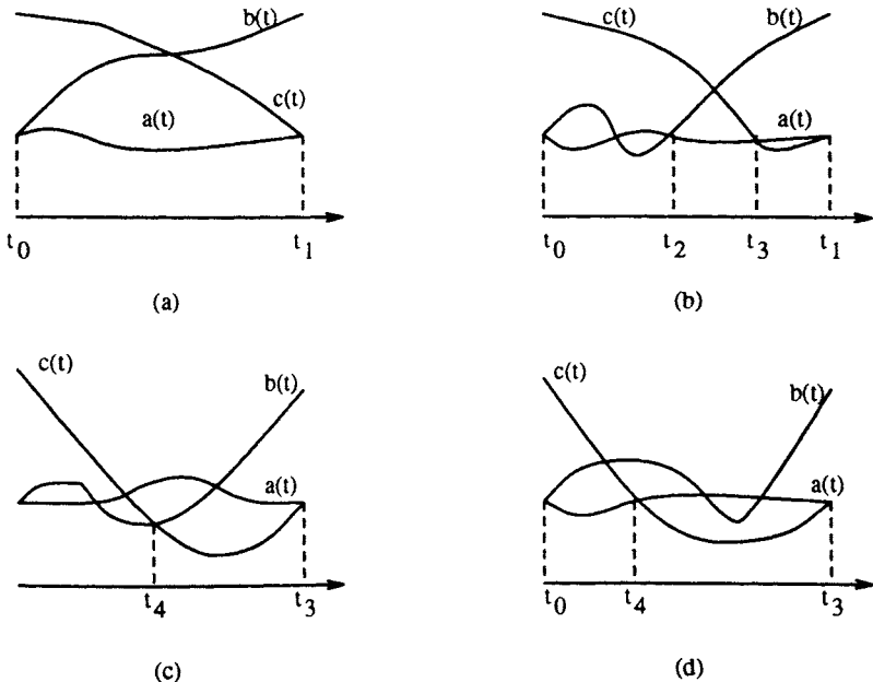
Fig. 6. Various cases in Claim 3.
