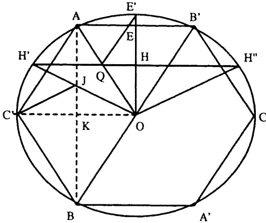
Fig. 7. Locating the point K in proof of upper bound.
