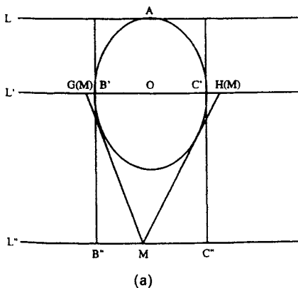
Fig. 1. Construction of \{A, B, C\} .
