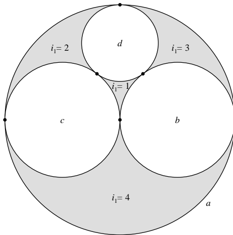
Fig. 4. Four lunes of Descartes quadruple.
