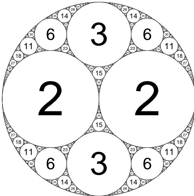
Fig. 1. The integral Apollonian circle packing (-1, 2, 2, 3) .
