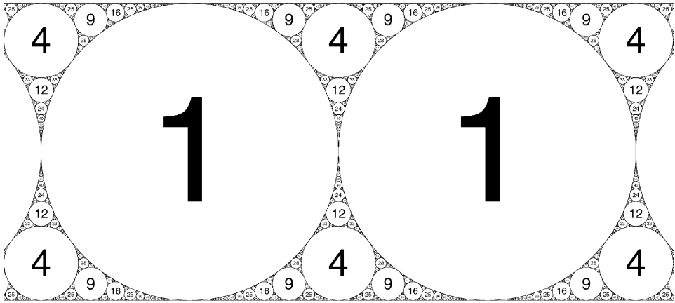
Fig. 2. The Apollonian circle packing (0, 0, 1, 1) .
