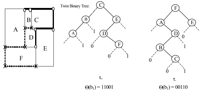
Fig. 9: Different representations for a slicing floorplan
