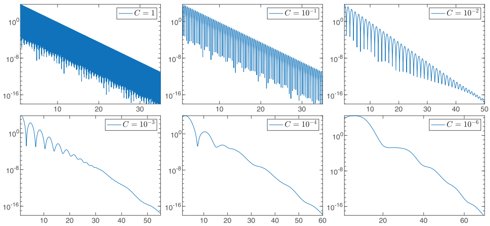
Figure 7. Error versus t along \eta = \overset{\circ}{\eta} = 0.5 exponential Bregman dynamics for Problem 4.1.
