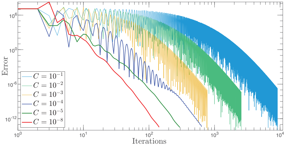
Figure 8. Discretization of the polynomial Bregman dynamics using PolyHTVI with different values of C for Problem 4.1 (without momentum restarting).
