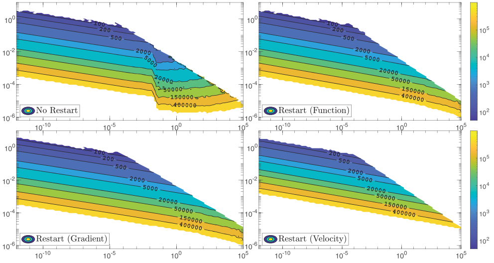
Figure 4. Contour plot of the number of iterations required to achieve convergence in the (C, h) -plane, for the p = \hat{p} = 8 PolyHTVI algorithm applied to Problem 4.1.
