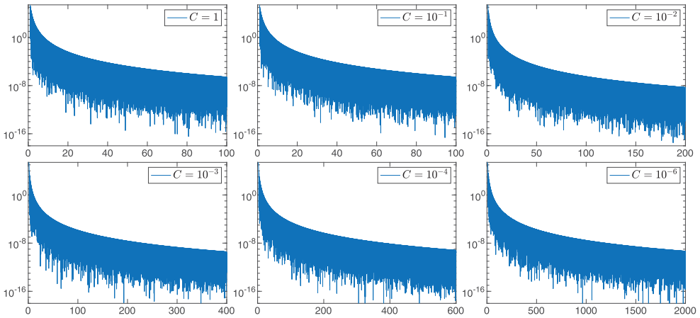
Figure 9. Error versus t along p = \hat{p} = 6 polynomial Bregman dynamics for Problem 4.4.
