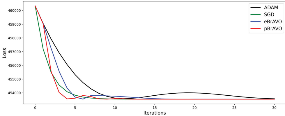
Figure 15. Comparison of algorithms applied to a Location Problem 4.7.
