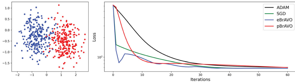
Figure 14. Comparison of algorithms applied to a Binary Classification Problem 4.6.
