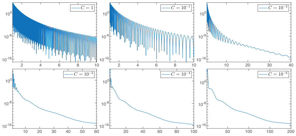
Figure 6. Error as a function of time t along the p = \overset{\circ}{p} = 6 polynomial Bregman dynamics for Problem 4.1, with different values of the constant C .
