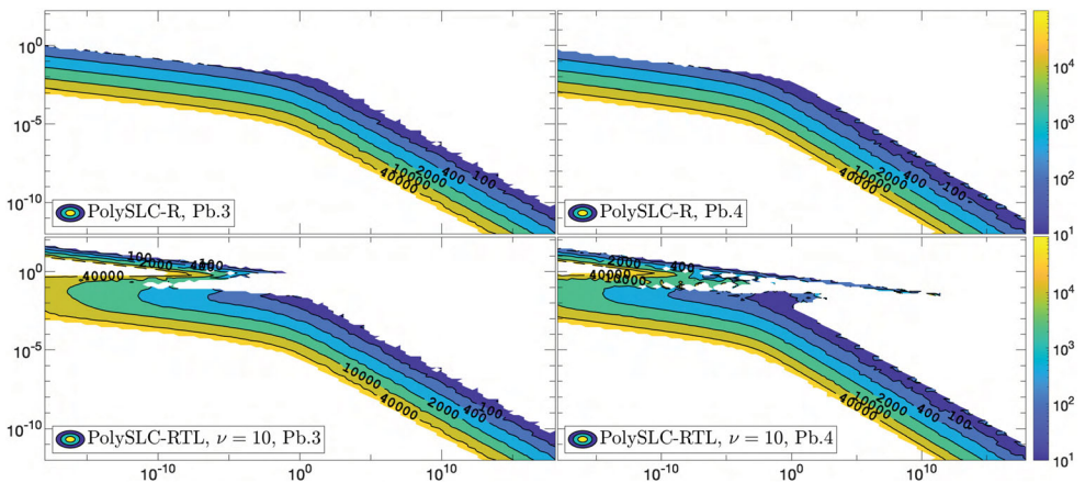
Figure 13. Contour plot of the number of iterations required to achieve convergence ( \delta = 10^{-8} ) in the (C, h) -plane, for the PolySLC-R and PolySLC-RTL algorithms, when applied with p = 10 to Problems 4.3 and 4.4.
