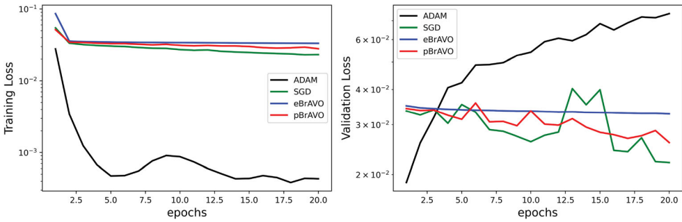
Figure 19. Evolution of the Binary Cross Entropy loss function on training and validation datasets for several algorithms, when applied to the Natural Language Processing problem of multi-label text classification of arXiv papers.
