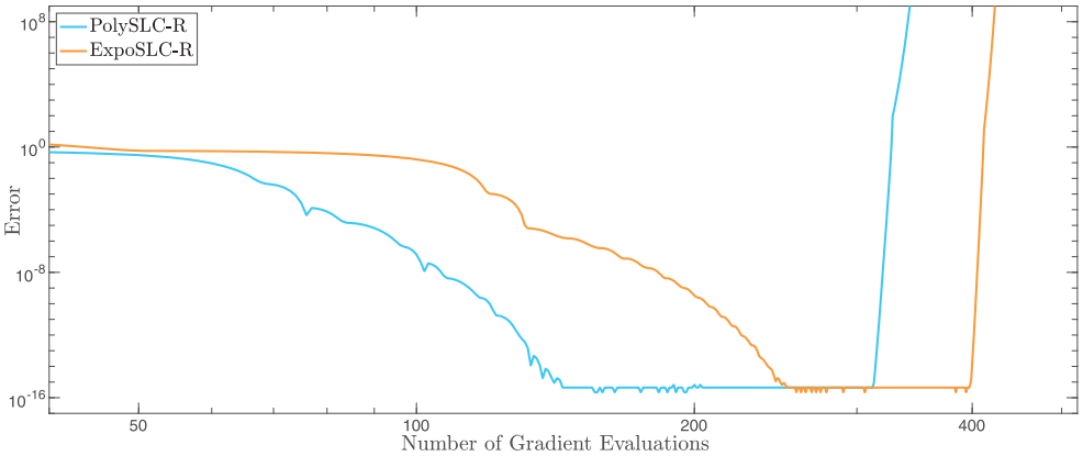
Figure 10. The PolySLC-R and ExpoSLC-R algorithms applied to Problem 4.2.
