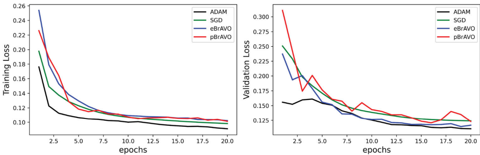
Figure 20. MSE evolution on training and validation datasets for several algorithms, when used to optimize an LSTM model for timeseries forecasting for weather prediction.
