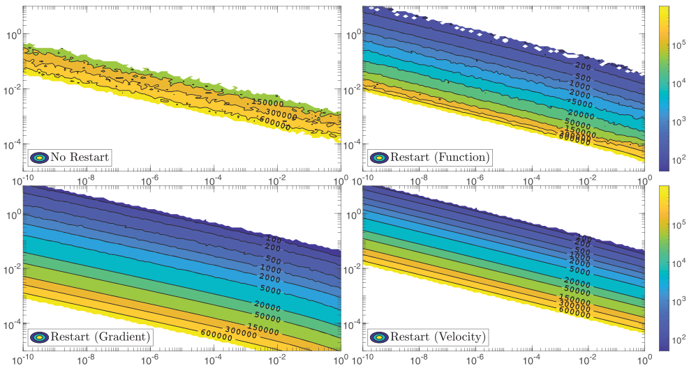
Figure 3. Contour plot of the number of iterations required to achieve convergence with \delta = 10^{-8} in the (C, h) -plane, for p = \hat{p} = 4 PolyHTVI applied to Problem 4.2.
