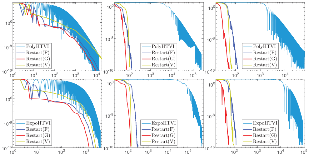
Figure 1. Error versus iterations number as the standard PolyHTVI and ExpoHTVI algorithms and their restarted versions (Function (F), Gradient (G) and Velocity (V)) are applied to Problem 4.1 (left), Problem 4.2 (middle) and Problem 4.3 (right).
