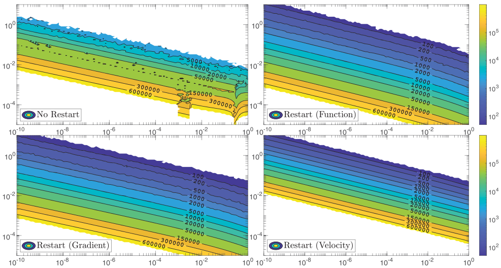
Figure 2. Contour plot of the number of iterations required to achieve convergence with \delta = 10^{-5} in the (C, h) -plane, for p = \hat{p} = 4 PolyHTVI applied to Problem 4.2.
