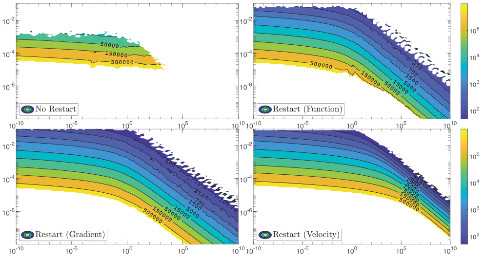
Figure 5. Contour plot of the number of iterations required to achieve convergence with \delta = 10^{-5} in the (C, h) -plane, for \eta = \hat{\eta} = 1 ExpoSLC applied to Problem 4.2.
