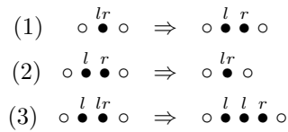
FIGURE 1. The three scattering rules. Filled-in sites are occupied. l denotes a left-mover, r a right-mover.
