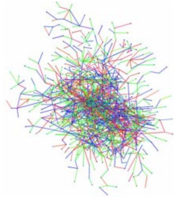
Figure 2: An induced subgraph of the collaboration graph G_1 .
