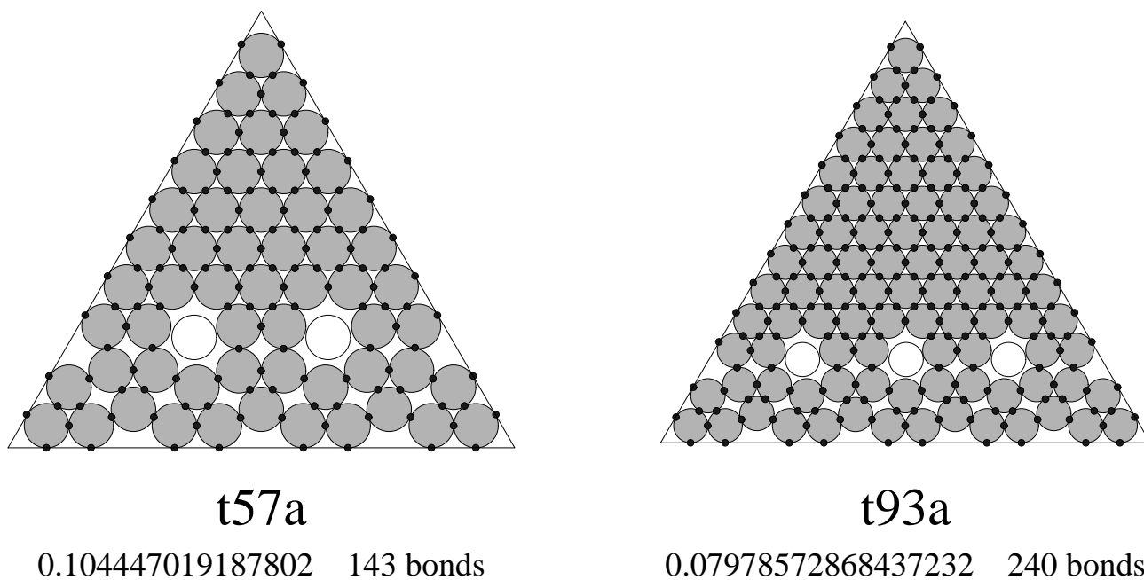
Figure 5.12: The best packings of 57 disks (t57a) and 93 disks (t93a).
