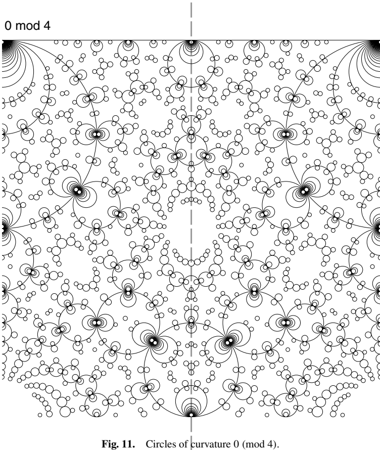
Fig. 11. Circles of curvature 0 (mod 4).
