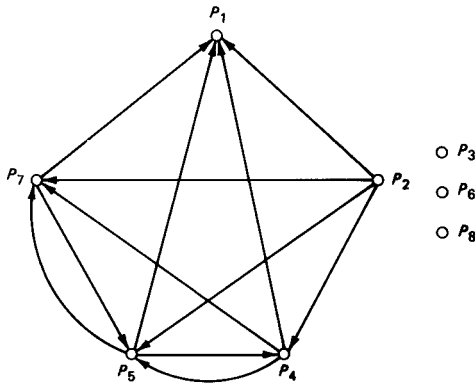
Fig. 6—Corresponding graph G for the Cardwell example. 6
