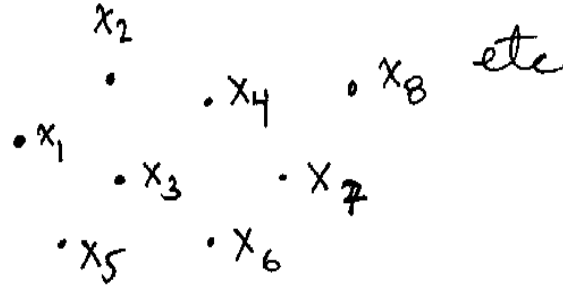
Fig. 14.2. Constructing a set with out an accumulation point.
