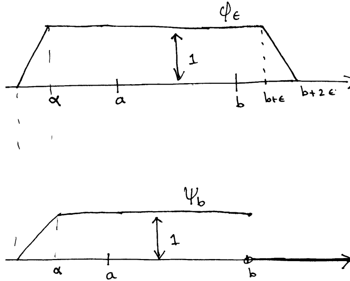
Fig. 30.5. A couple of functions in \overline{\mathcal{S}_c(\mathcal{A})} .
