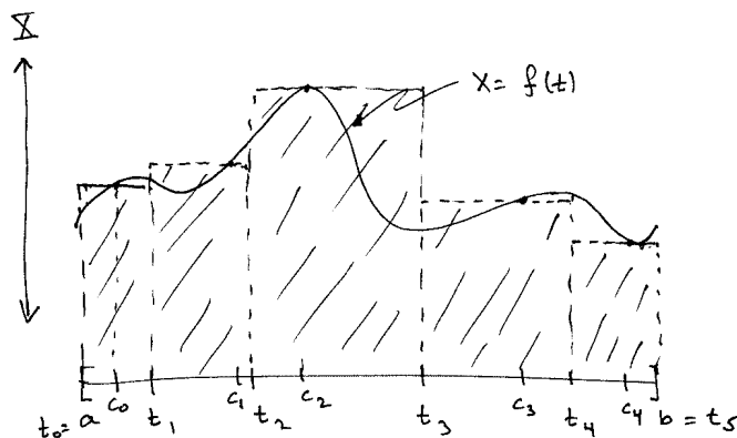
Fig. 10.1. The usual picture associated to the Riemann integral.
