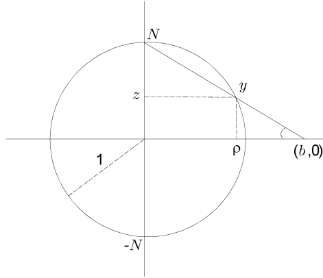
Fig. 15.7. Sterographic projection and the one point compactification of \mathbb{R}^n .
