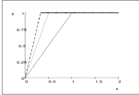
Fig. 18.3. Plots of \phi_1 , \phi_2 and \phi_3 .
