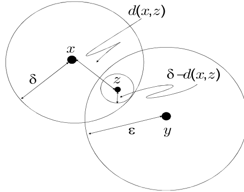
Fig. 13.2. Fitting balls in the intersection.
