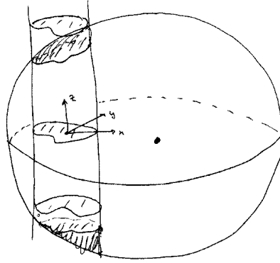
Fig. 36.3. The geometry of the solution to the wave equation in two dimensions.
