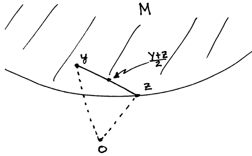
Fig. 8.2. The geometry of convex sets.
