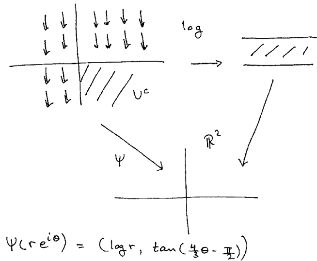
Fig. 11.2. Manufacturing vector fields where b(x) is discontinuous.
