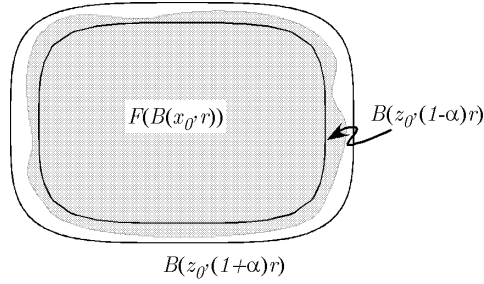
Fig. 12.1. Nesting of F(B(x_0, r)) between B(z_0, (1 - \alpha)r) and B(z_0, (1 + \alpha)r) .
