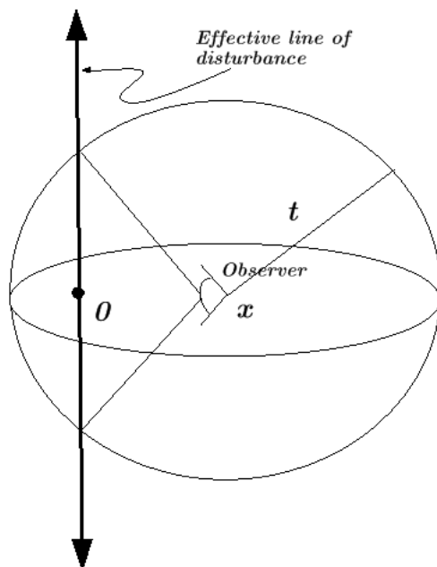
Fig. 35.2. The geometry of the solution to the wave equation in two dimensions. A flash at 0 \in \mathbb{R}^2 looks like a line of flashes to the fictitious 3-d observer and hence she sees the effect of the flash for t \geq |x| . The wave still propagates with speed 1. However there is no longer sharp propagation of the wave front, similar to water waves.
