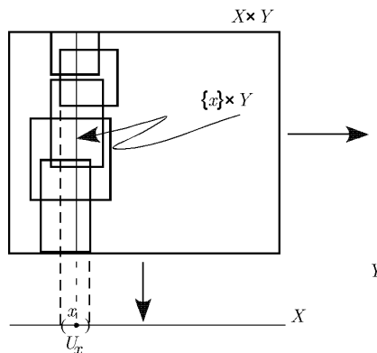
Fig. 14.4. Constructing the open set U_x .
