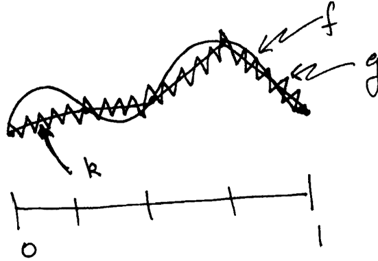
Fig. 16.1. Constructing a rough approximation, g , to a continuous function f .
