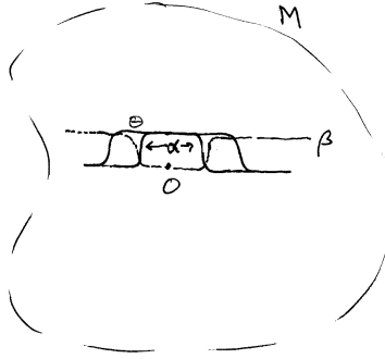
Fig. 35.3. The region M and the cutoff functions, \theta and \alpha .
