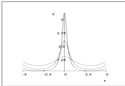
A plot of P_r(\delta) for r = 0.2, 0.5 and 0.7 .
