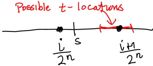
Fig. 25.1. The geometry of s and t with 2^{-(n+1)} < t - s \leq 2^{-n} .
