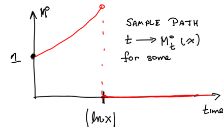
Fig. 28.2. A typical sample path of M_t^0(x) .
