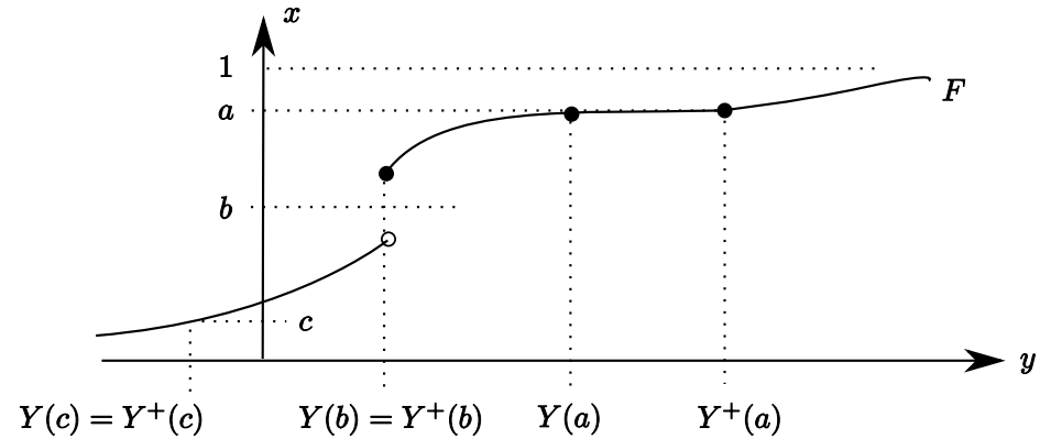
Fig. 21.3. The functions Y and Y^+ associated to F .
