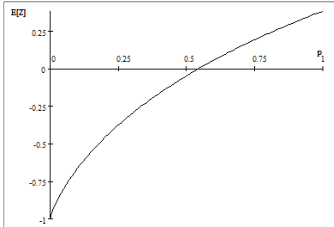
The graph of \mathbb{E}[\ln(p + U)] as a function of p . This function has a zero at p = p_c \cong 0.54221 .
