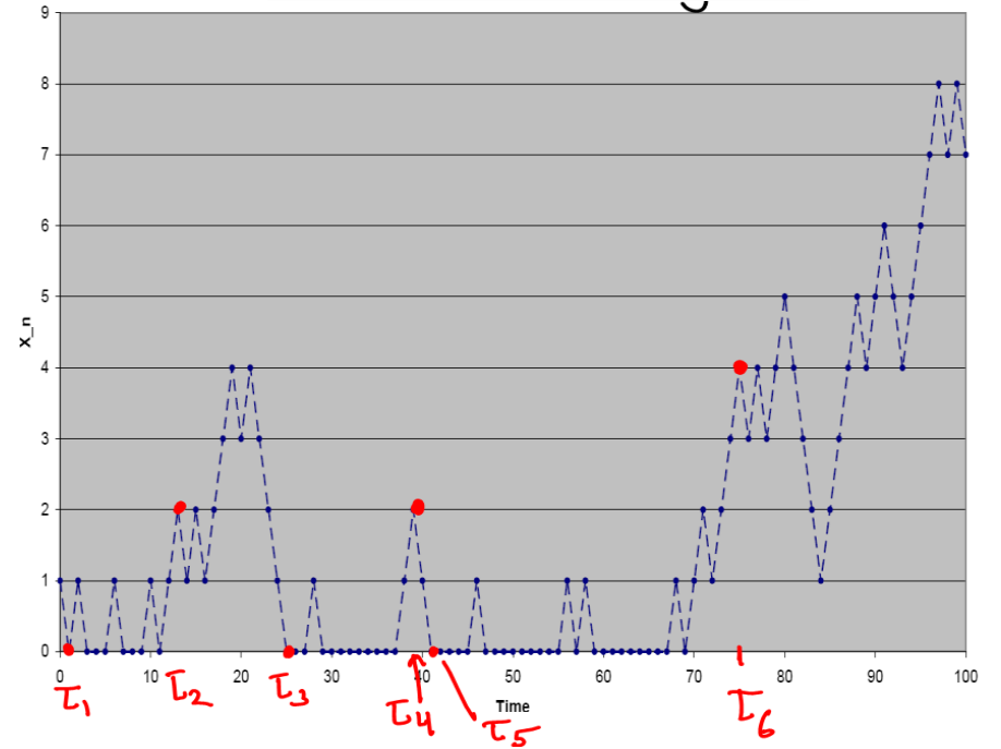
Fig. 18.2. A sample path of a positive submartingale along with stopping times \tau_{2j} and \tau_{2j+1} , successive hitting times of 2 and 0 respectively. Notice that X_{\tau_4 \wedge 70} - X_{\tau_3 \wedge 70} \geq 2 while X_{\tau_6 \wedge 70} - X_{\tau_5 \wedge 70} \geq 0 . Also observe that X_{\tau_8 \wedge 90} - X_{\tau_7 \wedge 90} = 0 .
