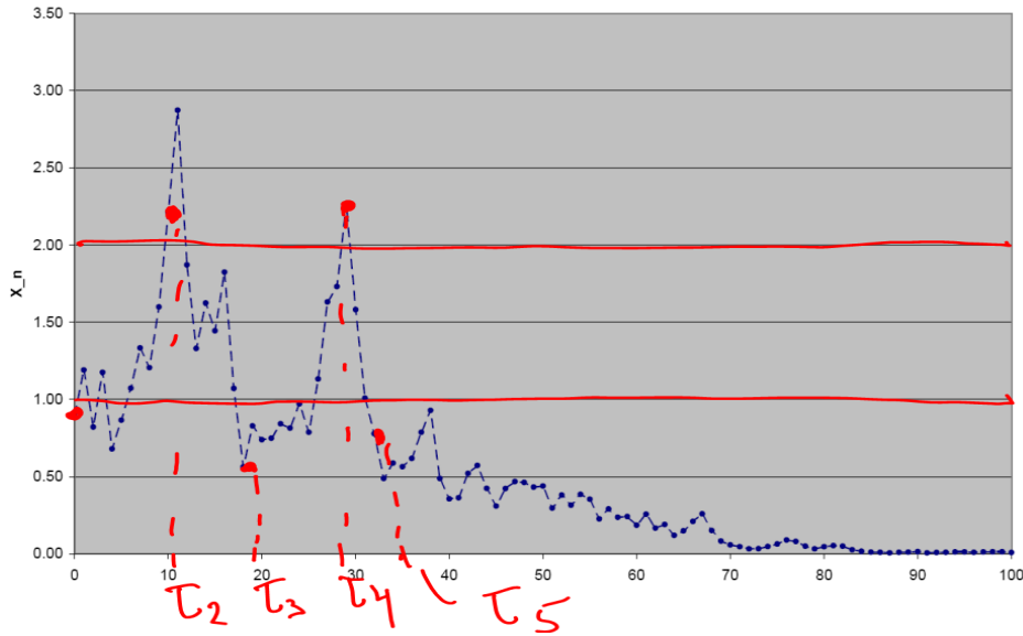
Fig. 18.1. A sample path of a positive martingale with crossing levels, a = 1 and b = 2 marked off.
