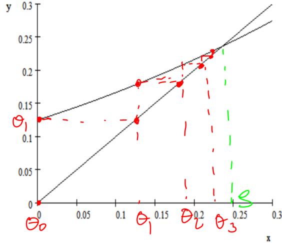
Fig. 19.2. The graphical interpretation of \theta_m = \varphi(\theta_{m-1}) starting with \theta_0 = 0 .
