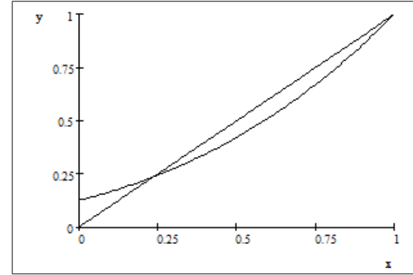
Fig. 19.1. Figure associated to \varphi(s) = \frac{1}{8}(1 + 3s + 3s^2 + s^3) which is relevant for Exercise 3.13 of Durrett on p. 249. In this case \rho \cong 0.23607 .
