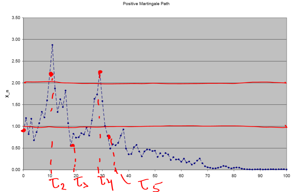
Fig. 18.1. A sample path of a positive martingale with crossing levels, a = 1 and b = 2 marked off.
