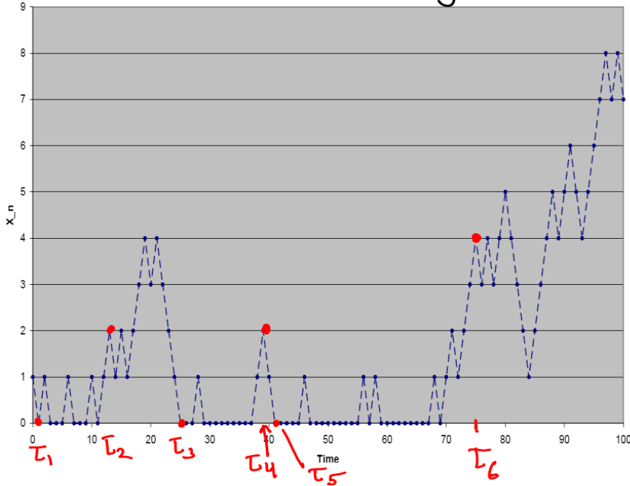
Fig. 18.2. A sample path of a positive submartingale along with stopping times \tau_{2j} and \tau_{2j+1} , successive hitting times of 2 and 0 respectively. Notice that X_{\tau_4 \wedge 70} - X_{\tau_3 \wedge 70} \geq 2 while X_{\tau_6 \wedge 70} - X_{\tau_5 \wedge 70} \geq 0 . Also observe that X_{\tau_8 \wedge 90} - X_{\tau_7 \wedge 90} = 0 .
