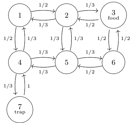
Fig. 17.3. The jump diagram for our proverbial rat in the maze.
