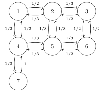
Fig. 17.1. The jump diagram for our proverbial rat in the maze.
