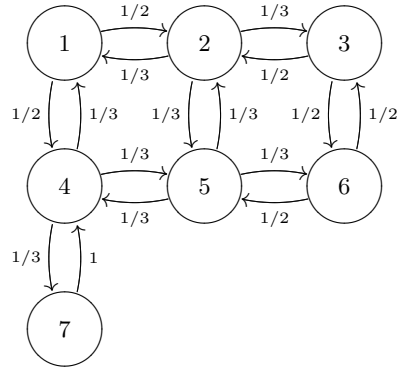
Fig. 17.1. The jump diagram for the rat in the maze.
