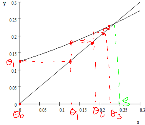
Fig. 18.2. The graphical interpretation of \theta_m = \varphi(\theta_{m-1}) starting with \theta_0 = 0 .
