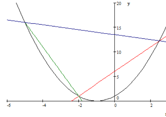
Fig. 12.3. A convex function along with three chords corresponding to x_0 = -5 and x_1 = -2 , x_0 = -2 and x_1 = 5/2 , and x_0 = -5 and x_1 = 5/2 with slopes, m_1 = -15/3 , m_2 = 15/6 and m_3 = -1/2 respectively. Notice that m_1 \leq m_3 \leq m_2 .
