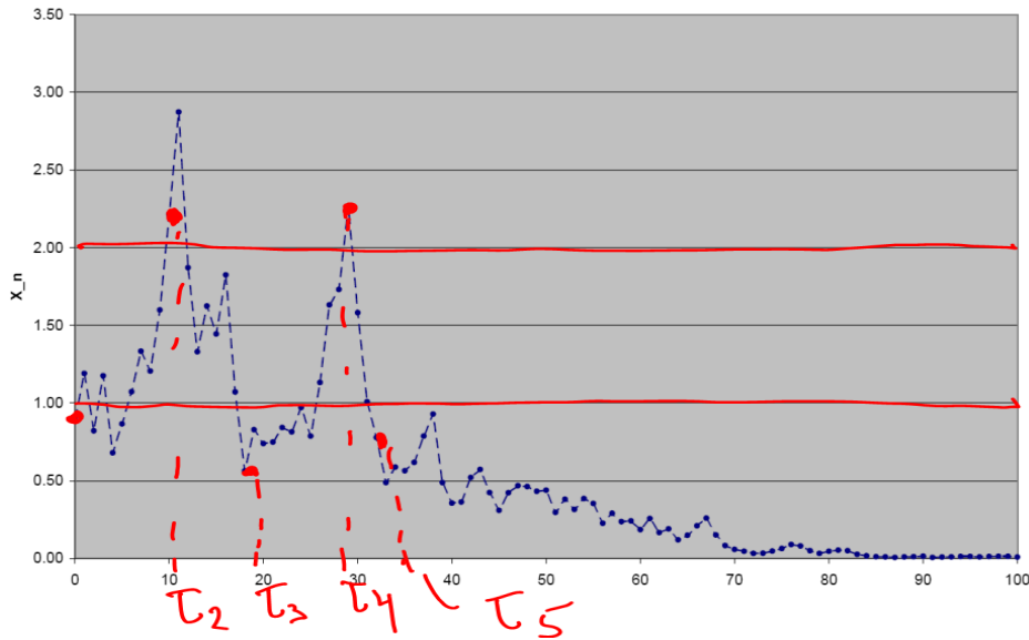
Fig. 17.1. A sample path of a positive martingale with crossing levels, a = 1 and b = 2 marked off.
