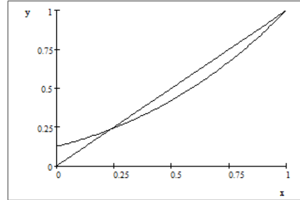
Fig. 18.1. Figure associated to \varphi(s) = \frac{1}{8}(1 + 3s + 3s^2 + s^3) which is relevant for Exercise 3.13 of Durrett on p. 249. In this case \rho \cong 0.23607 .
