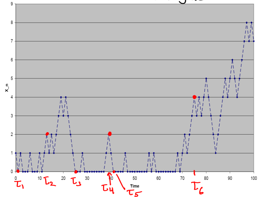
Fig. 17.2. A sample path of a positive submartingale along with stopping times \tau_{2j} and \tau_{2j+1} , successive hitting times of 2 and 0 respectively. Notice that X_{\tau_4 \wedge 70} - X_{\tau_3 \wedge 70} \geq 2 while X_{\tau_6 \wedge 70} - X_{\tau_5 \wedge 70} \geq 0 . Also observe that X_{\tau_8 \wedge 90} - X_{\tau_7 \wedge 90} = 0 .
