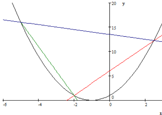
Fig. 12.3. A convex function along with three cords corresponding to x_0 = -5 and x_1 = 5/2 , and x_0 = -5 and x_1 = 5/2 with slopes, m_1 = -15/3 , m_2 = 15/6 and m_3 = -1/2 respectively. Notice that m_1 \leq m_3 \leq m_2 .
