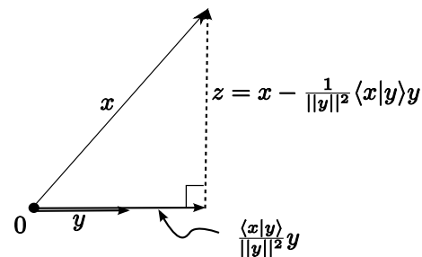
Fig. 13.1. The picture behind the proof of the Schwarz inequality.
