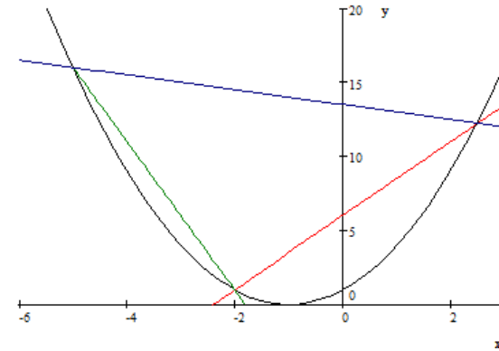
Fig. 12.3. A convex function along with three cords corresponding to x_0 = -5 and x_1 = -2 , x_0 = -2 and x_1 = 5/2 , and x_0 = -5 and x_1 = 5/2 with slopes, m_1 = -15/3 , m_2 = 15/6 and m_3 = -1/2 respectively. Notice that m_1 \leq m_3 \leq m_2 .
