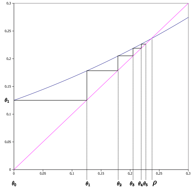
Fig. 19.3. The graphical interpretation of \theta_m = \varphi(\theta_{m-1}) starting with \theta_0 = 0 . ■
