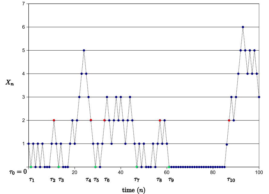
Fig. 18.4. A sample path of a positive submartingale along with stopping times \tau_{2j-1} and \tau_{2j} which are the successive hitting times of 0 and 2 respectively. If we take N = 70 in this case, then observe that X_{\tau_8 \wedge 70} - X_{\tau_7 \wedge 70} \geq 2 while X_{\tau_{10} \wedge 70} - X_{\tau_9 \wedge 70} = 0
