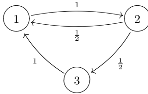
Fig. 17.6. A simple 3 state jump diagram.
