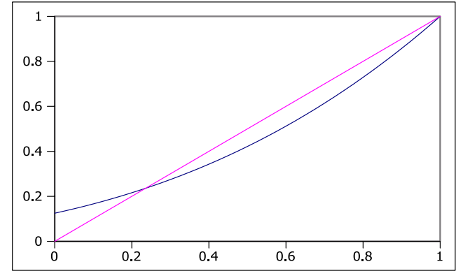
Fig. 19.1. Figure associated to \varphi(s) = \frac{1}{8}(1 + 3s + 3s^2 + s^3) which is relevant for Exercise 3.13 of Durrett on p. 249. In this case \rho \cong 0.23607 .
