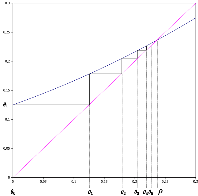
Fig. 19.2. The graphical interpretation of \theta_m = \varphi(\theta_{m-1}) starting with \theta_0 = 0 .
