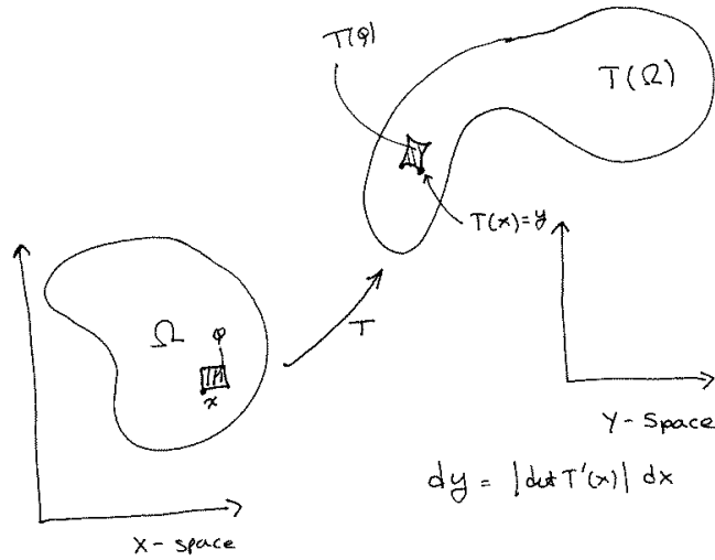
Fig. 20.1. The geometric setup of Theorem \frac{\text{t. 20.19}}{20.19} .
