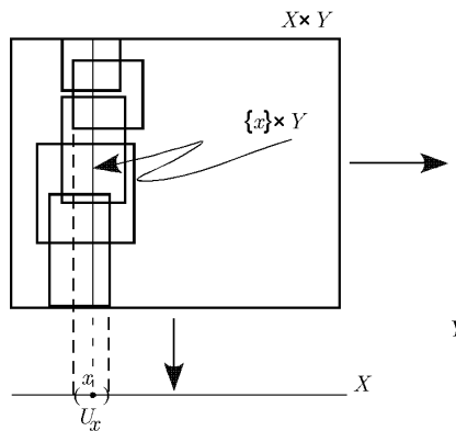
Fig. 14.4. Constructing the open set U_x . \boxed{\text{f. 14.4}}
