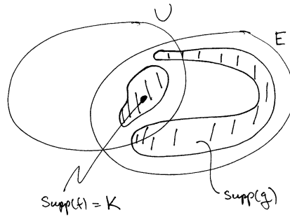
Fig. 31.1. Constructing a function g which approximates 1_{E \setminus U} . \boxed{\text{f.30.1}}
