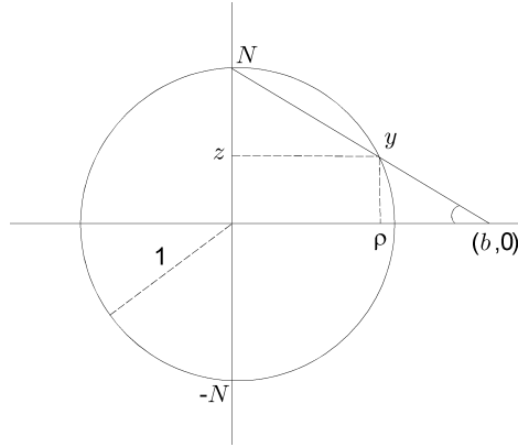
Fig. 15.7. Sterographic projection and the one point compactification of \mathbb{R}^n . f.15.8
