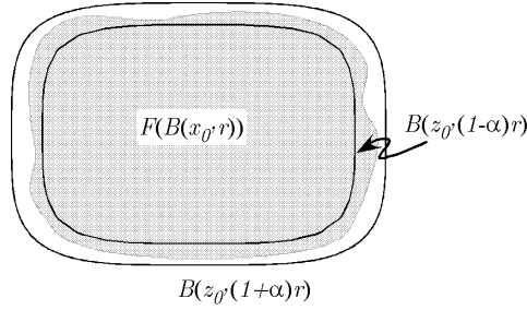
Fig. 12.1. Nesting of F(B(x_0, r)) between B(z_0, (1 - \alpha)r) and B(z_0, (1 + \alpha)r) . f. 12.1
