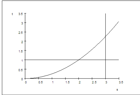
Fig. 5.1. A picture proof of Proposition p.5.3 .
