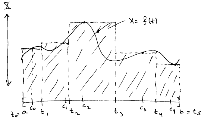
Fig. 10.1. The usual picture associated to the Riemann integral. f.10.1
