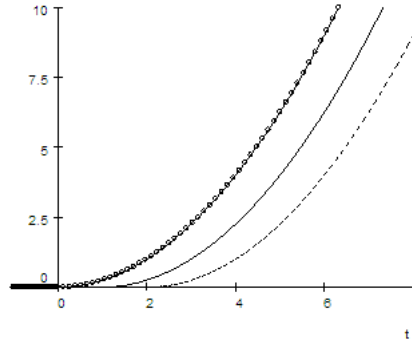
Fig. 11.1. Three different solutions to the ODE \dot{y}(t) = |y(t)|^{1/2} with y(0) = 0 . f.11.1
