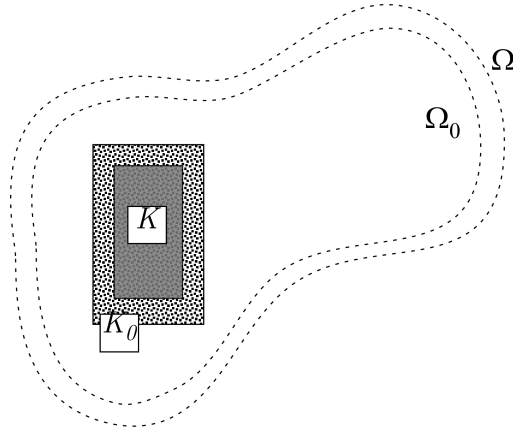
Fig. 26.1. The geometry of K \subset K_0 \subset \Omega_0 \subset \Omega .
