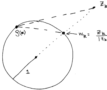
Fig. 24.1. Sliding points to the unit circle.
