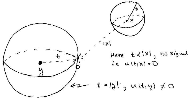
Fig. 36.2. The geometry of the solution to the wave equation in three dimensions. \boxed{\text{f.35.2}}
