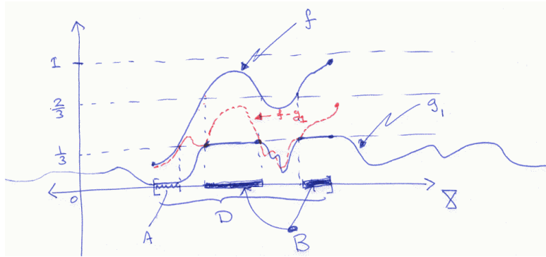
Fig. 7.1. Reducing f by subtracting off a globally defined function g_1 \in C(X, [0, \frac{1}{3}]) . \boxed{\text{f.7.1}}
