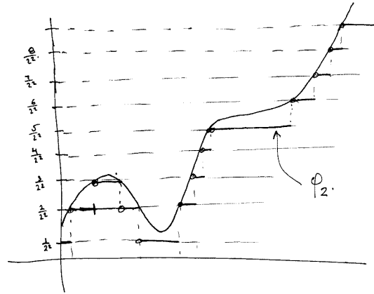
Fig. 18.2. Constructing simple functions approximating a function, f : X \rightarrow [0, \infty] . f. 18.2
