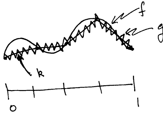
Fig. 16.1. Constructing a rough approximation, g , to a continuous function f . f.16.1
