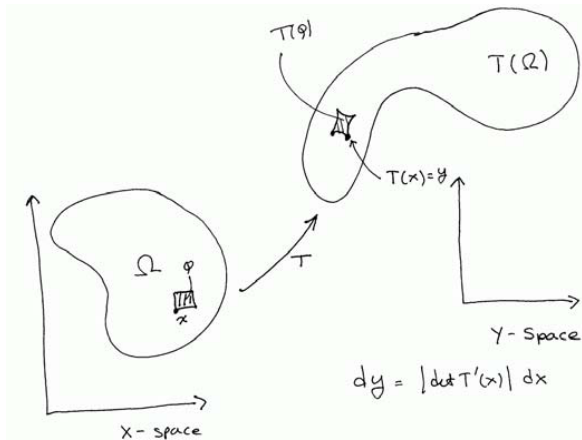
Fig. 20.1. The geometric setup of Theorem 20.19.
