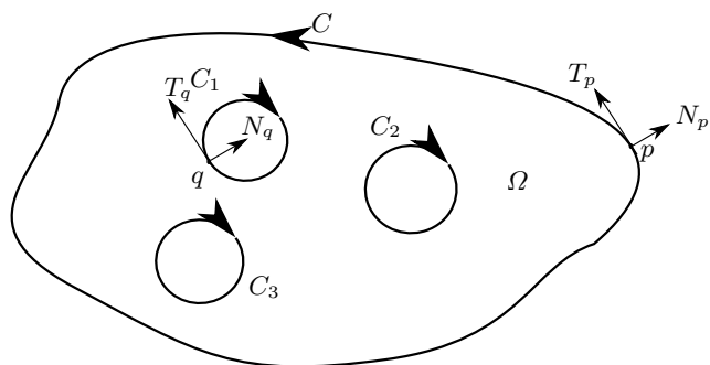
Fig. 14.2. The region \Omega whose oriented boundaries are shown as C_1 \cup C_2 \cup C_3 \cup C . The orientation on the boundaries are determined by finding the outward pointing normals and then using the right hand rule.
