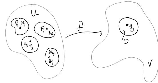
Fig. 11.5. Here we suppose that q is a regular value and f^{-1}(\{q\}) is a set of size 4.
