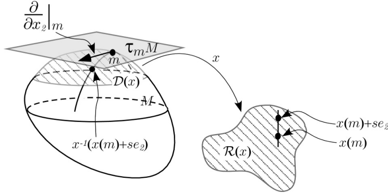
Fig. 13.4. Forming a basis of tangent vectors.
