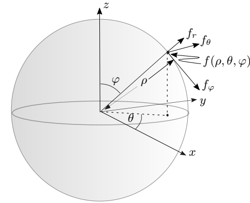
Fig. 15.2. The solid \rho -ball with boundary. From this picture one sees that \{f_r, f_\theta, f_\varphi\} forms an orthogonal set with \|f_r\| = 1 , \|f_\theta\| = \rho \sin \varphi , and \|f_\varphi\| = \rho . Moreover, \{f_r, f_\theta, f_\varphi\} satisfies the left hand rule and therefore it follows that \det[f_r | f_\theta | f_\varphi]_{(r, \theta, \varphi)} = -\rho^2 \sin \varphi .
