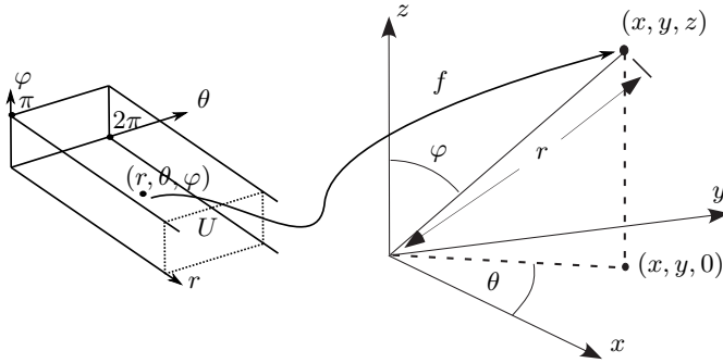
Fig. 15.1. This picture depicts the spherical parametrization of (most) of \mathbb{R}^3 .
