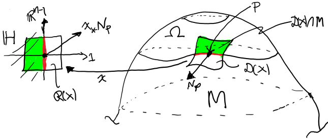
Fig. 14.1. A region, \Omega \subset M , which is a manifold with boundary. We have also depicted an outward pointing normal at the point p \in \partial\Omega .
