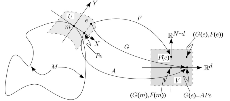
Fig. 13.2. Constructing charts for M using the inverse function theorem. For simplicity of the drawing, m \in M is assumed to be the origin of E = X \oplus Y .
