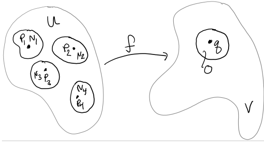
Fig. 11.5. Here we suppose that q is a regular value and f^{-1}(\{q\}) is a set of size 4.
