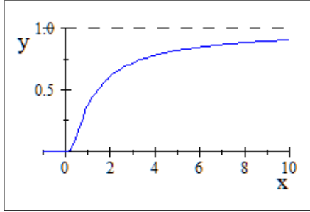
Fig. 11.1. Plot of y = f(x) .
