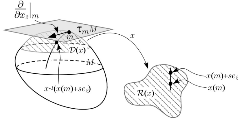
Fig. 13.4. Forming a basis of tangent vectors.
