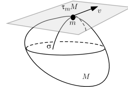
Fig. 13.3. Tangent plane, \tau_m M , to M at m and a vector, v , in \tau_m M .
