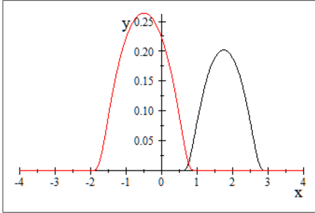
Fig. 11.3. Here is the plots for \varphi_{0.5,3} (black) and \varphi_{-2,1} (red).
