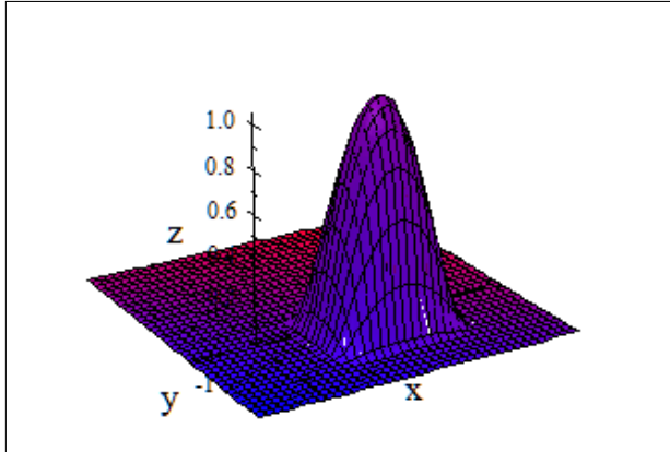
Fig. 11.4. Plot of 20 \cdot \varphi_R(x, y) where R = (-\frac{1}{2}, 3) \times (-2, 1) .
