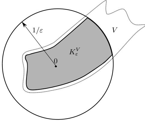
Fig. 10.2. The shaded area indicates K_\varepsilon^V where as W_\varepsilon^V is the region K_\varepsilon^V with its boundary removed.
