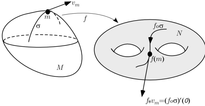
Fig. 13.5. The differential of f .
