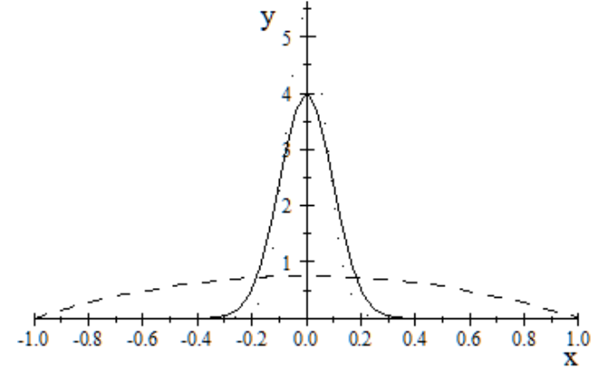
Fig. B.1. A plot of q_1 , q_{50} , and q_{100} . The most peaked curve is q_{100} and the least is q_1 . The total area under each of these curves is one.
