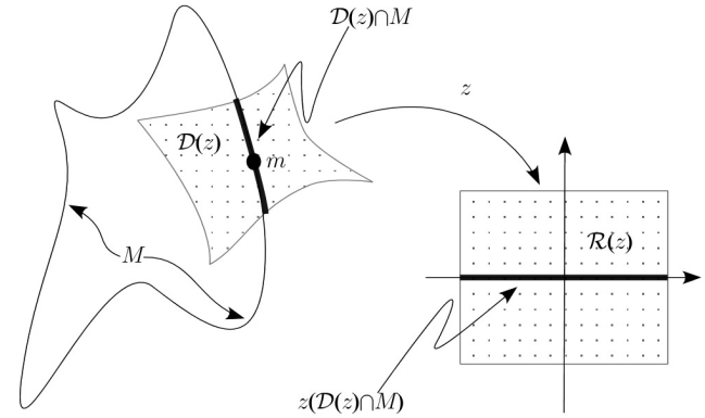
Fig. 13.1. An imbedded one dimensional submanifold in \mathbb{R}^2 .
