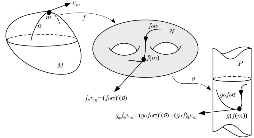
Fig. 13.6. The chain rule.
