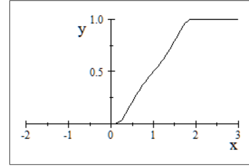
Fig. 11.2. This is a plot of the function, H_2(x) = f(x) / (f(x) + f(x-2)) .
